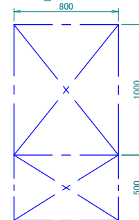
ARROW VIEW B INSPECTION DOOR (CEILING OPENING)
